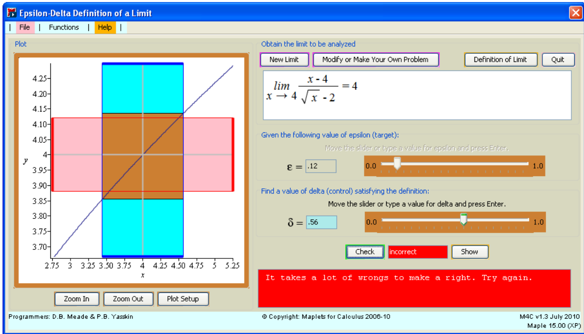
Figure E.7 Screen shot of the Epsilon-Delta Continuity Maplelet after using 'check' feature
